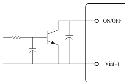
Fig. 2 Open Collector Enable Circuit
