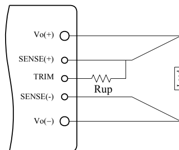
Fig. 5 Circuit to Increase Output Voltage
