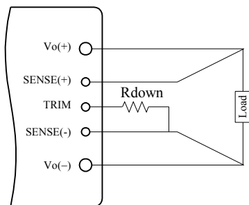
Fig. 6 Circuit to Decrease Output Voltage
